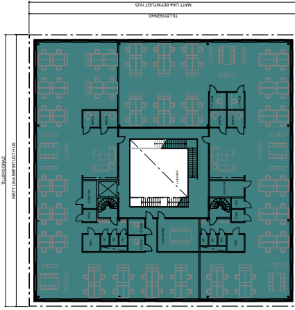
Plan 3: 1170 m 2
