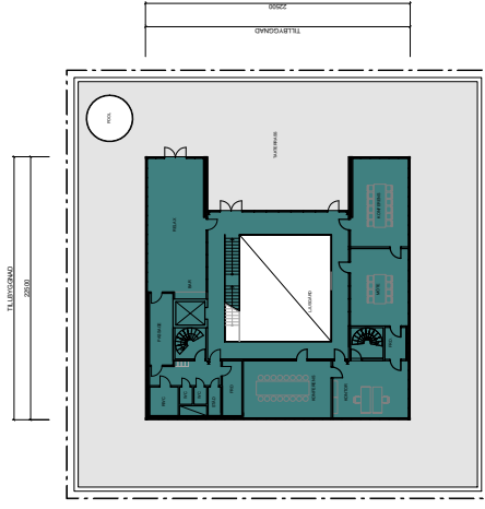
Plan 5: 380 m 2
